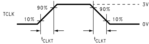
FIGURE 4. Serializer Input Clock Transition Time
